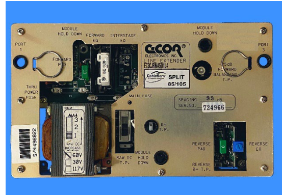
CableServ Flex Net E7 series Mid/High-Split Upgrade
