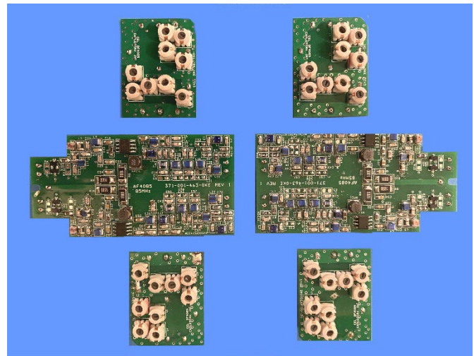
CableServ OA4444S Upgrade Mid-Split Kit
