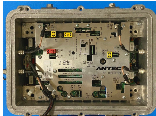
CableServ FTMB 1 GHz Mid/High Split
