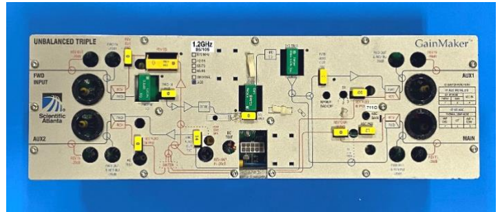
CableServ UBT, BT, HGDL, LGDL 1.2 GHz Upgrade
