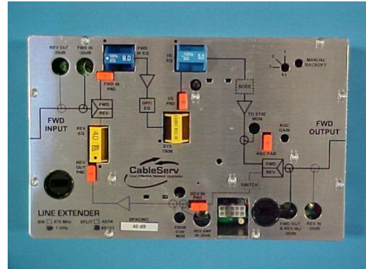
CableServ GainMaker LE Forward and Reverse Upgrade
