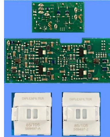
CableServ Cisco GM LE Band-Split Kit
